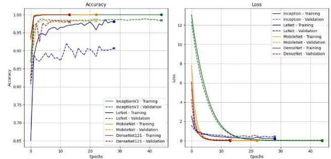
Fig. 8. Accuracy and loss curves during training for yawning state detection using LeNet, DenseNet121, InceptionV3 and MobileNet architectures.
