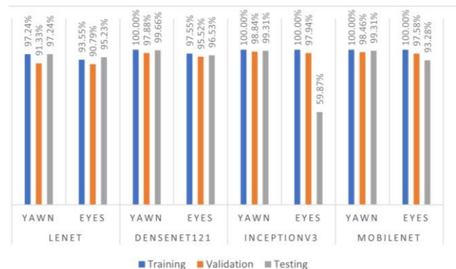
Fig. 10. Comparative performance of CNN architectures in the training, validation and testing phases for yawning and eye states.
