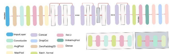
Fig. 5. Structure of the DenseNet121 architecture with optimization techniques.
